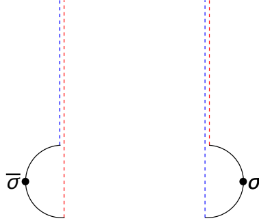
Figure 17: Pictorial representation of the anti-flag state \bar{\sigma}^\perp (left) and the flag state \mathbb{L}\sigma (right). \mathbb{L}\sigma is defined with the insertion of [\sigma(0)]^{\frac{\ell}{2}h} on the right half disc of diameter \ell , where h is the conformal map (15.27) and \frac{\ell}{2} is a rescaling factor, and glued to an infinitesimally thin semi-infinite strip, whose left edge (dashed blue) and right edge (dashed red, shifted upward by \ell ) are identified with the two halves of the open string similarly to the sliver map (Figure 16).
