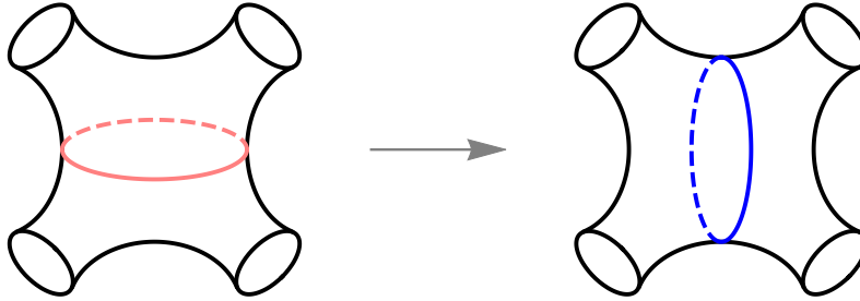
Figure 27: The crossing move relating two different pair-of-pants decompositions of the four-holed sphere.
