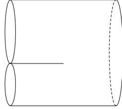
Figure 23: The lightcone gauge worldsheet diagram representing the tree-level 2 \rightarrow 1 amplitude.
