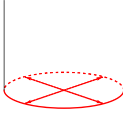
Figure 21: The cross cap state |\otimes\rangle is produced by the identification (17.6) on the cylinder parameterized by w \sim w + 2\pi with \text{Im}(w) \geq 0 .
