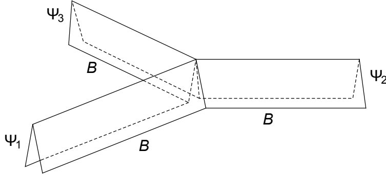
Figure 14: The cubic open string vertex with three open string propagators attached. Here B represents the boundary of the worldsheet, whereas the open string states \Psi_i propagate along the folded strips.
