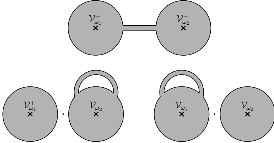
Figure 18: Degeneration limit of worldsheet diagrams that leads to logarithmic divergences due to propagation of the open string collective modes (e.g. on a \mathbb{Z}\mathbb{Z} -instanton considered in section 16.2). Formally, the divergences cancel in the sum of the three diagrams, but finite ambiguities remain in the on-shell approach.
