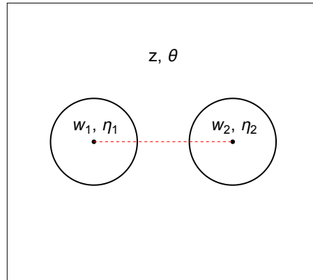
Figure 9: The superplane with a pair of R punctures.
