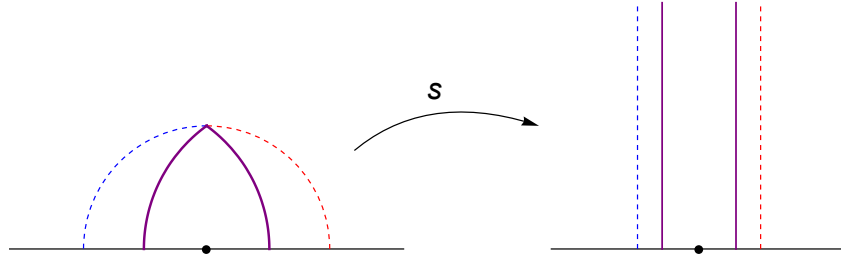
Figure 16: The sliver map u = s(z) \equiv \frac{2}{\pi} \arctan(z) takes the upper half unit z -disc (left) to the semi-infinite strip |\text{Re}(u)| \leq \frac{1}{2} on the UHP (right). The wedge bounded by purple curves on the left is mapped to the semi-infinite strip between the vertical purple lines on the right.
