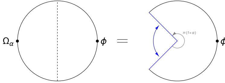
Figure 15: The BPZ inner product between the wedge state \Omega_\alpha and a general state \phi (transformed into the disc coordinate via the conformal map h ) is equivalent to the 1-point function of \phi on the cone-shaped disc \tilde{D}^2 with deficit angle 2\pi(1 - \frac{1+\alpha}{2}) .
