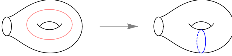
Figure 28: The crossing move relating two different pair-of-pants decompositions of the one-holed torus.
