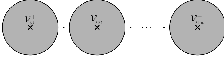
Figure 19: Worldsheet diagram that computes the leading non-perturbative correction to the closed string 1 \rightarrow n amplitude, of order e^{-S_{ZZ}} , mediated by a single ZZ-instanton.
