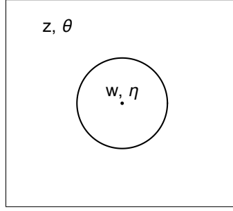
Figure 8: The superplane with an NS puncture.
