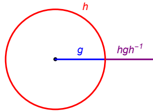
Figure 30: The action of \hat{h} on a defect operator (black dot) in \mathcal{H}_g , realized by encircling with \mathcal{L}_h (red) and a 4-way junction.
