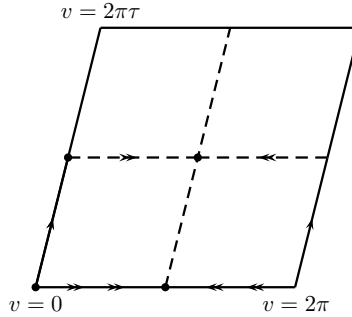
Figure 25: The pillow geometry is the quotient T^2/\mathbb{Z}_2 . The four points on the plane 0, z, 1, \infty are mapped to the \mathbb{Z}_2 fixed points w = 0, \pi, \pi(\tau + 1), \pi\tau respectively.
