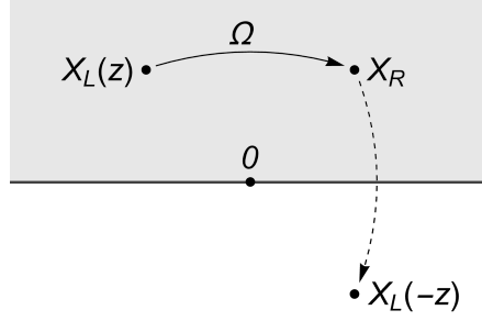
Figure 22: The action of the worldsheet parity \Omega represented through the doubling trick.
