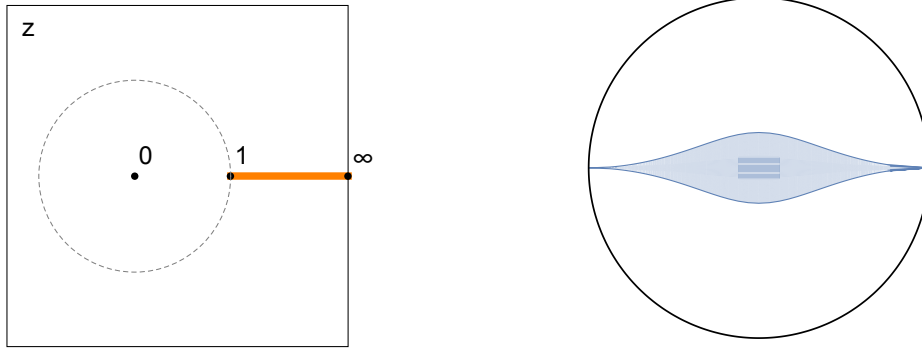
Figure 26: The complex z -plane with a branch cut along [1, \infty) is mapped to the eye-shaped region on the unit q disc. The Virasoro conformal block can be analytically continued to the entire q disc.
