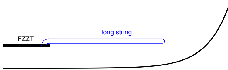
Figure 13: A high energy open string ending on an FZZT-brane in the asymptotic region, whose midpoint approaches the Liouville wall.
