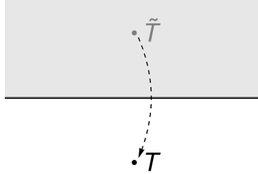
Figure 11: Starting from the upper half plane with a conformal boundary condition, the doubling extends the holomorphic stress-energy tensor to the lower half plane via the identification T(z' = \bar{z}) = \tilde{T}(\bar{z}) , \text{Im}(z) > 0 .
