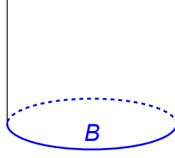
Figure 12: The boundary state |B\rangle is created by the boundary condition B on the cylinder parameterized by w \sim w + 2\pi with \text{Im}(w) \geq 0 .
