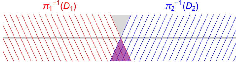
Figure 10: The uplifted patches \pi_1^{-1}(D_1) and \pi_2^{-1}(D_2) generally do not agree along D_1 \cap D_2 . The integrals along the fibers of \pi_1 and \pi_2 must be supplemented by the integration over the interpolating patch, shown in gray (with positive orientation) and purple (with negative orientation).
