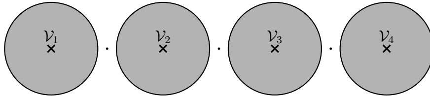
Figure 20: The leading D-instanton contribution to the four supergraviton amplitude is represented by the worldsheet diagram consisting of four discs, all of which are subject to the same D-instanton boundary condition labeled by (x, \theta) .
